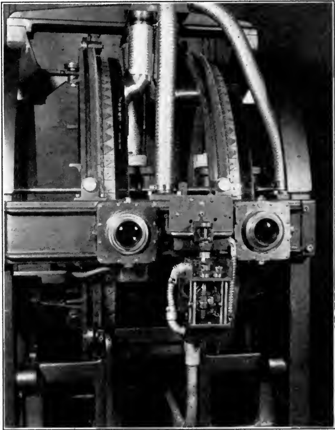
FIG. 1. General view of front of automatic slide projector, showing double projector system.
